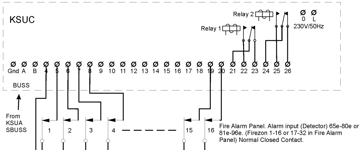
Connection of a fire alarm panel.
