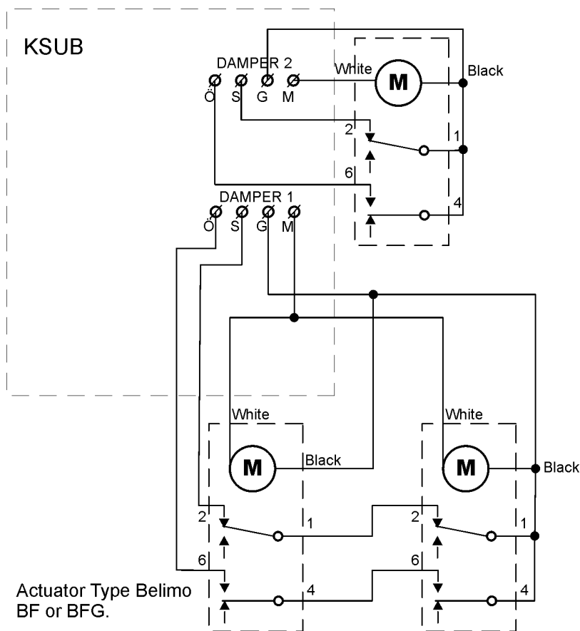
Parallel connection of damper at connection DAMPER 1 and single connection at DAMPER 2.
